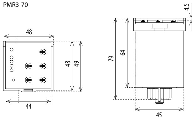
PMR3-70
